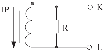
Built-in with sampling resistance voltage output type
