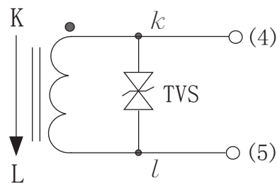
Built-in two-way protection diode current output type
